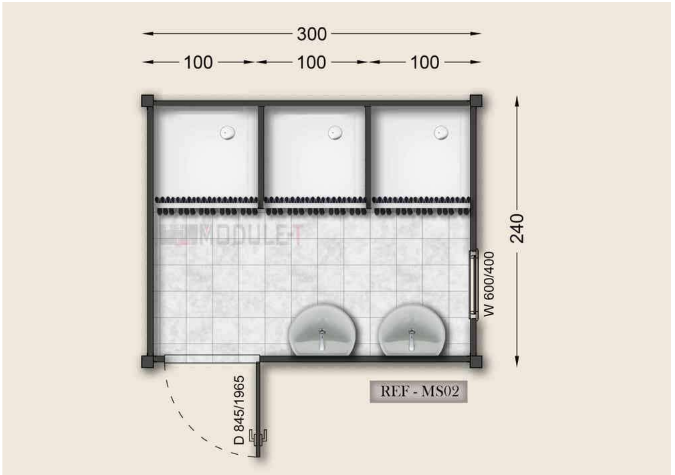
Shower container 3,00x2,40m
